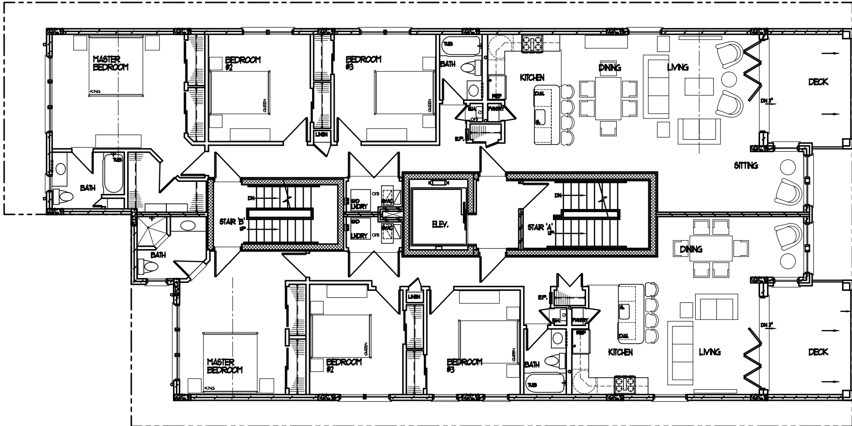
SECOND FLOOR PLAN SCALE: 3/16" = 1'-0"
